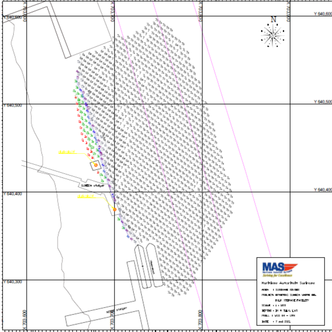
Figure 1: Depth survey SUHOZA White Oil Bulk Storage Facility May 2021 (depths are referred to LWS)
