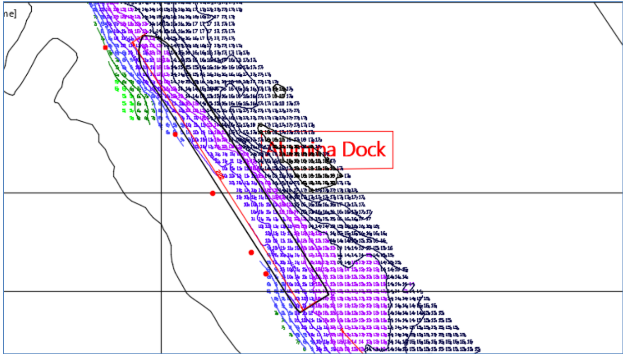
Figure 1: Depth survey Alumina Dock July 2020 (depths are referred to LWS)
