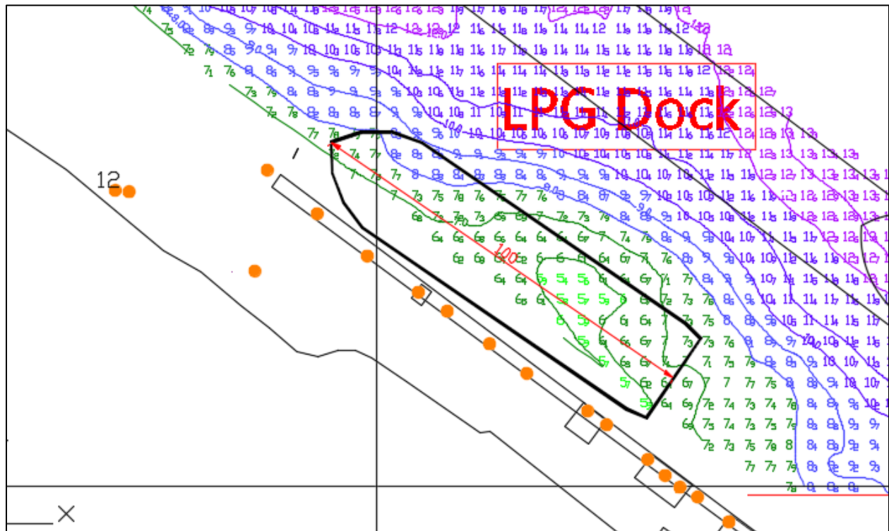
Figure 1: Depth survey LPG Dock July 2020 (depths are referred to LWS)
